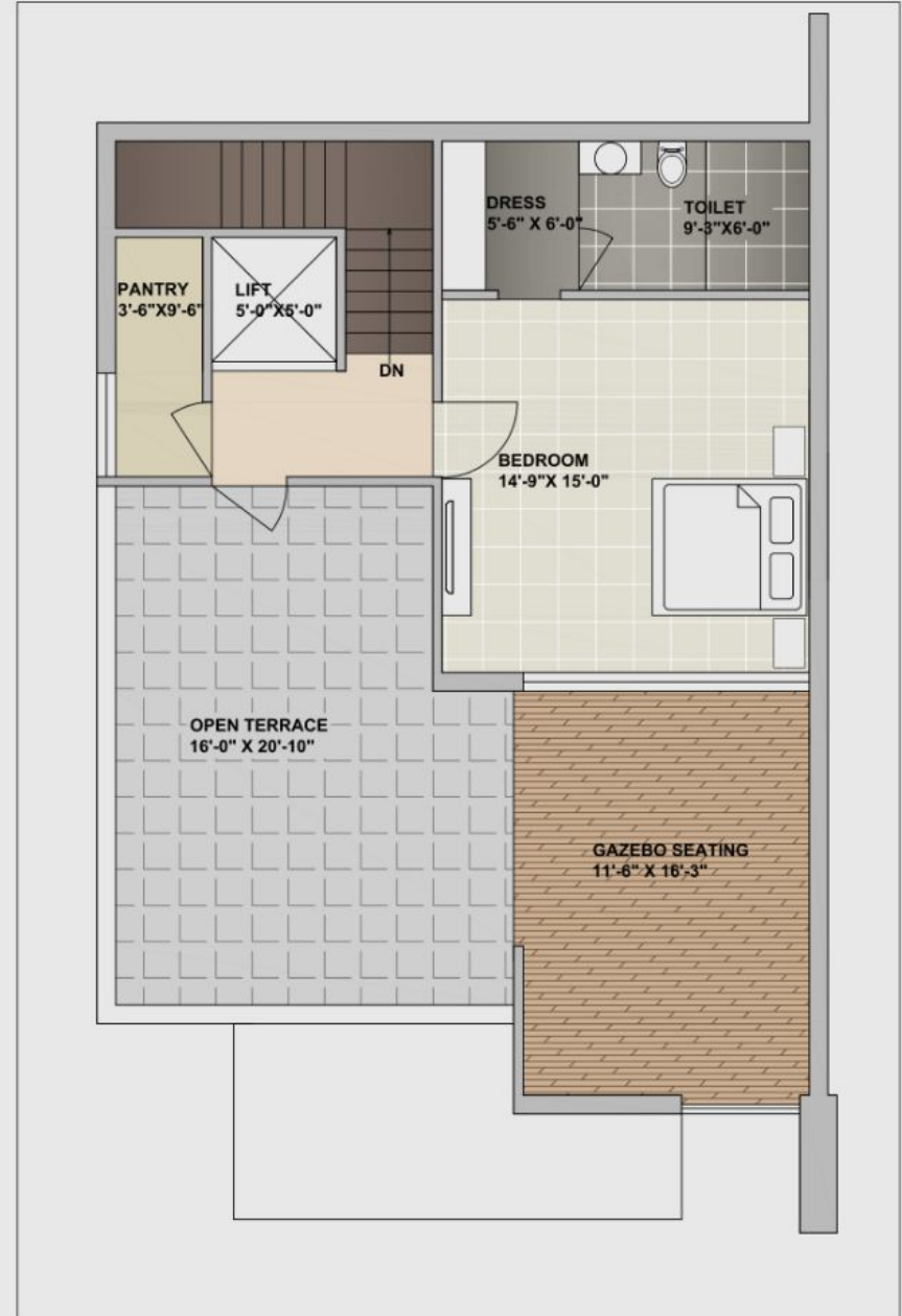
THIRD FLOOR PLAN (TYPE - A)
