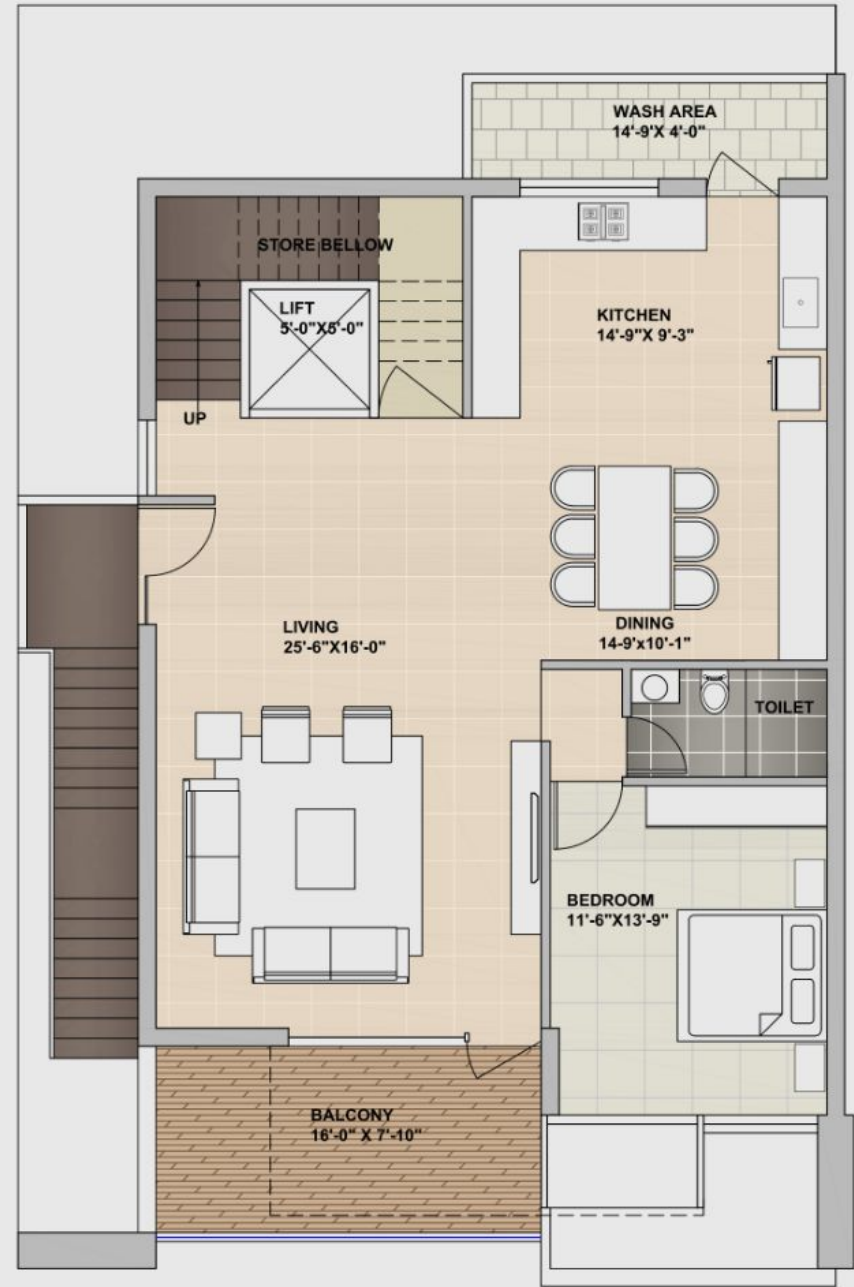
FIRST FLOOR PLAN (TYPE - A)
